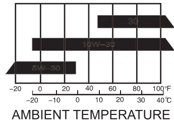
SAE VISCOSITY GRADES
